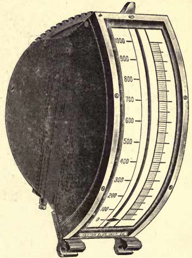
Fig. 121.—Weston Permanent-Magnet Ammeter (Edgewise pattern)
